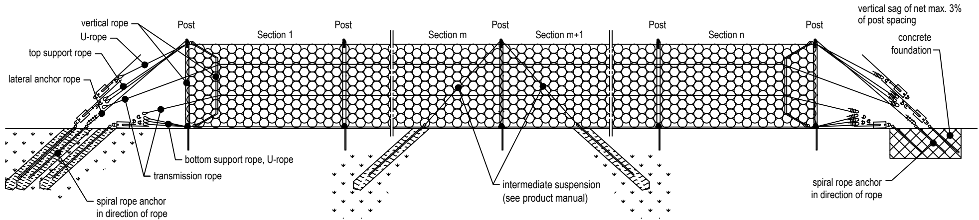
layout of anchor points (details see product manual RXE-3000)
