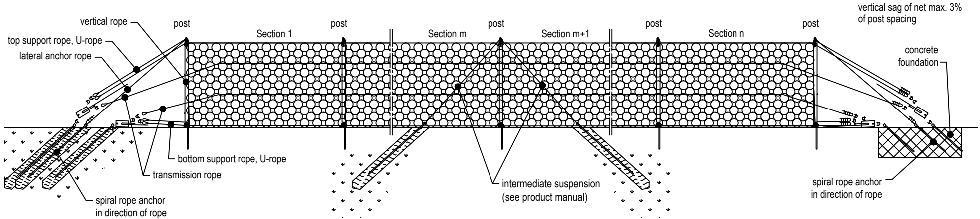
layout of anchor points (details see product manual RXE-1000)
