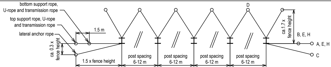
layout of anchor points (details see product manual RXE-1000)
