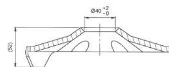
Section B-B
